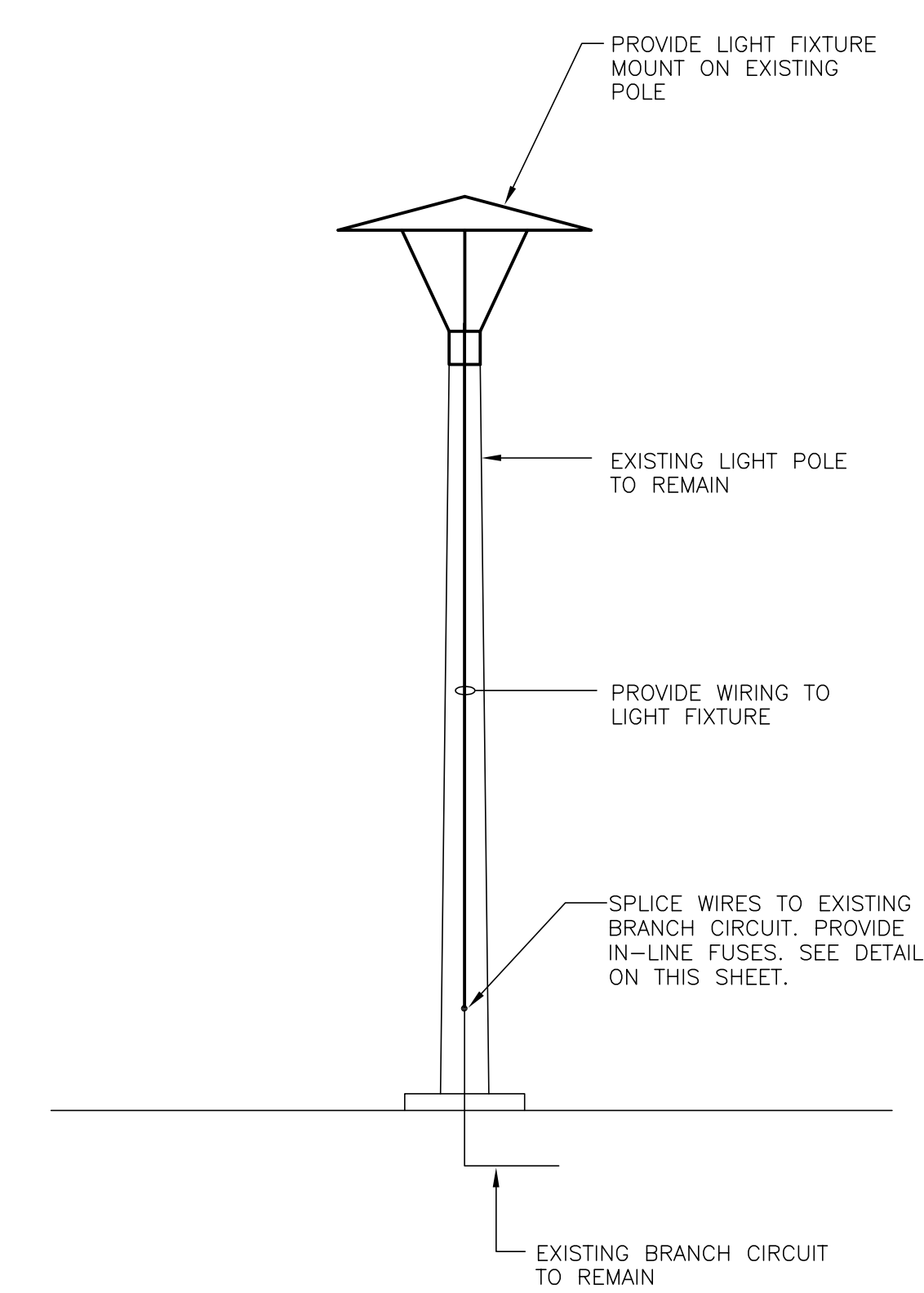
PARKING LOT POLE - NEW WORK
