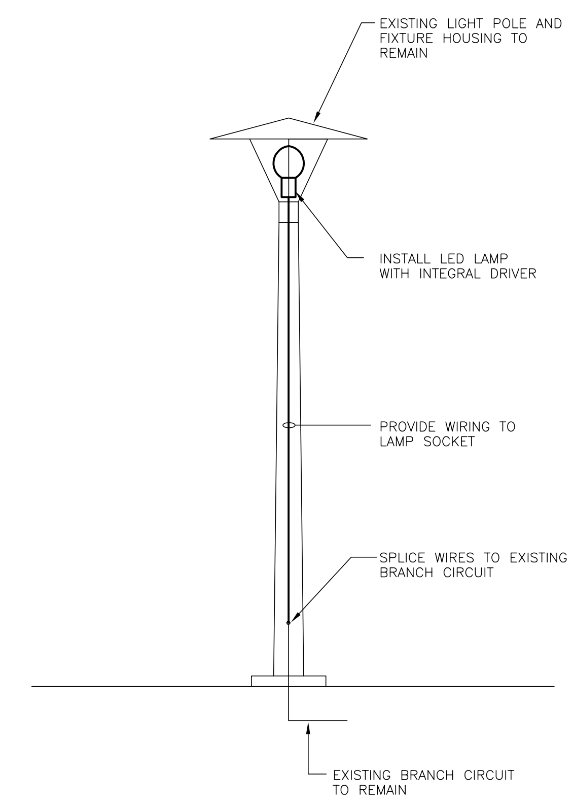
PEDESTRIAN POLE - NEW WORK
