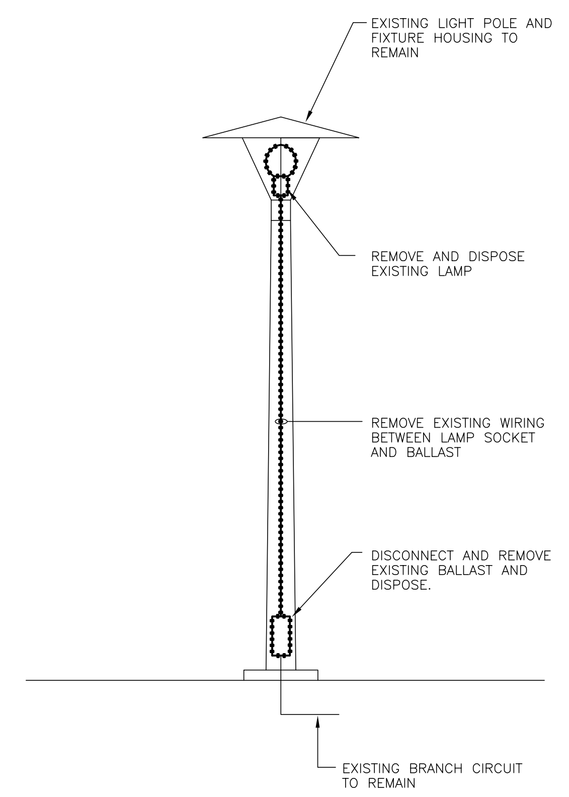
PEDESTRIAN POLE - DEMOLITION
