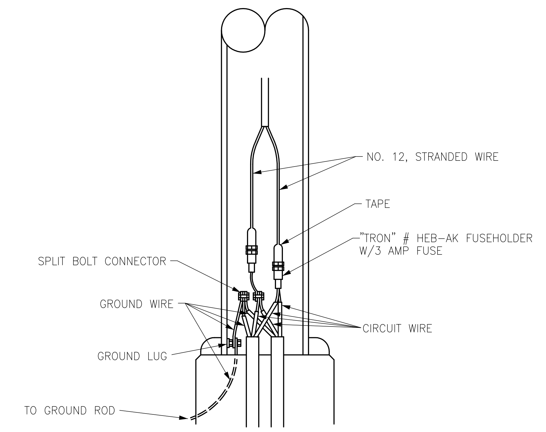
CONDUCTOR CONNECTIONS DETAIL
