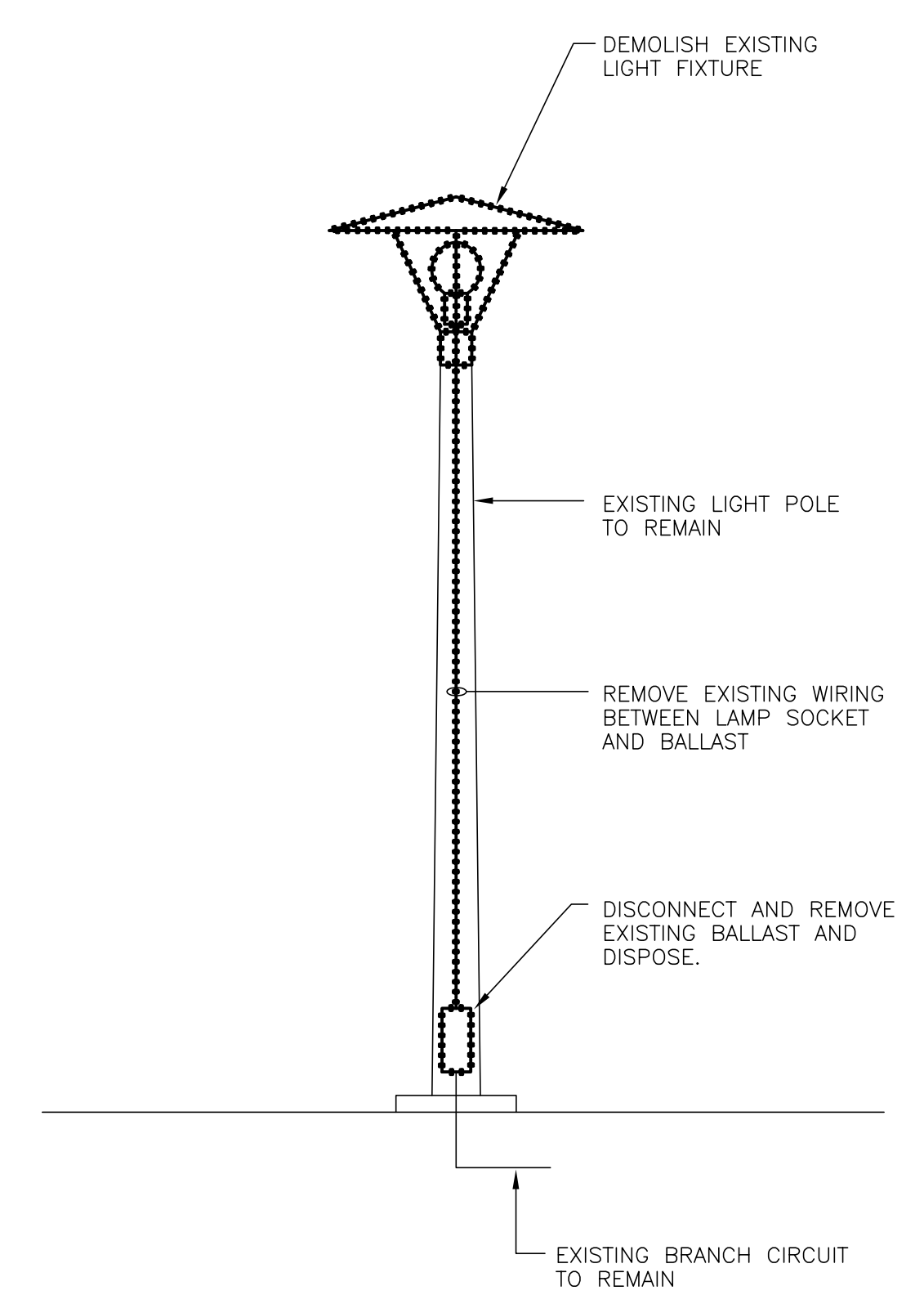
PARKING LOT POLE - DEMOLITION
